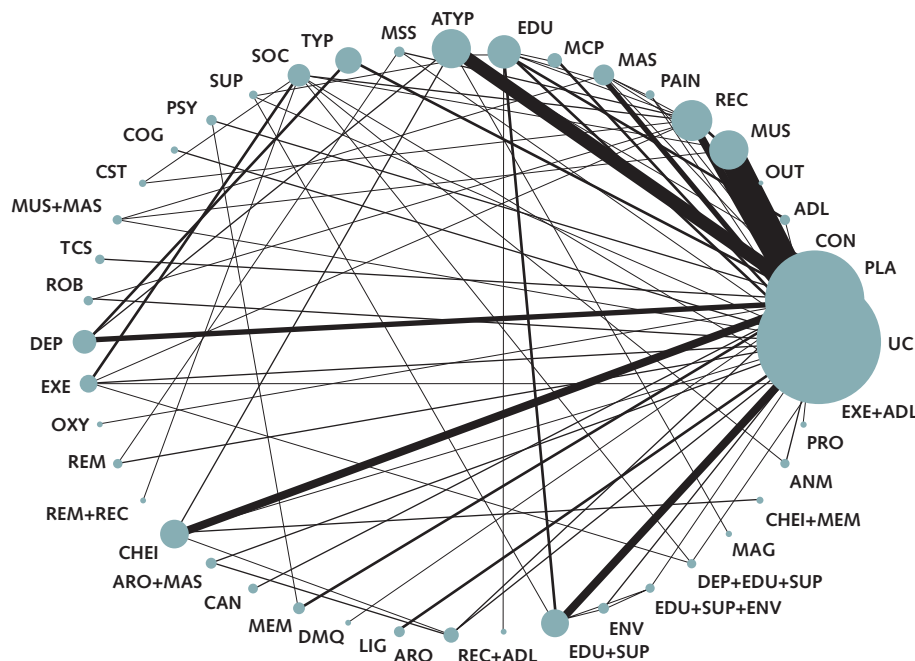
Figure 2. Network diagrams for network of interventions targeted at the combined outcome of agitation and aggression in persons with dementia.
